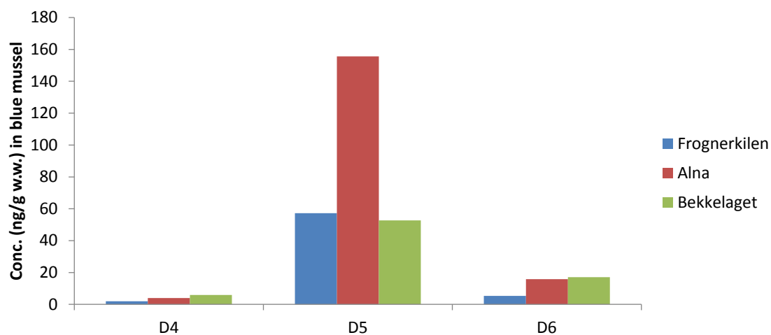
Figure 30. Concentrations of cyclic volatile methylsiloxanes (ng/g wet wt.) in polychaetes (A.) and blue mussel (B.) from Frognerkilen, the mouth of Alna River and at Bekkelaget. One composite sample per station.
