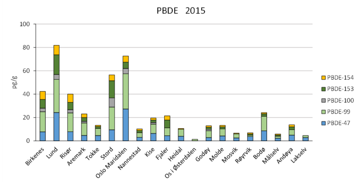
Figure 9: Distribution of selected PBDE congeners (without BDE-209) from the 2015 study.
