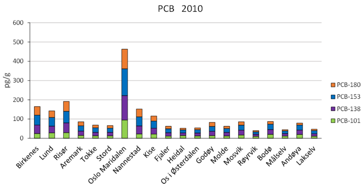
Figure 2: Distribution of selected PCB congeners from the 2010 study.
