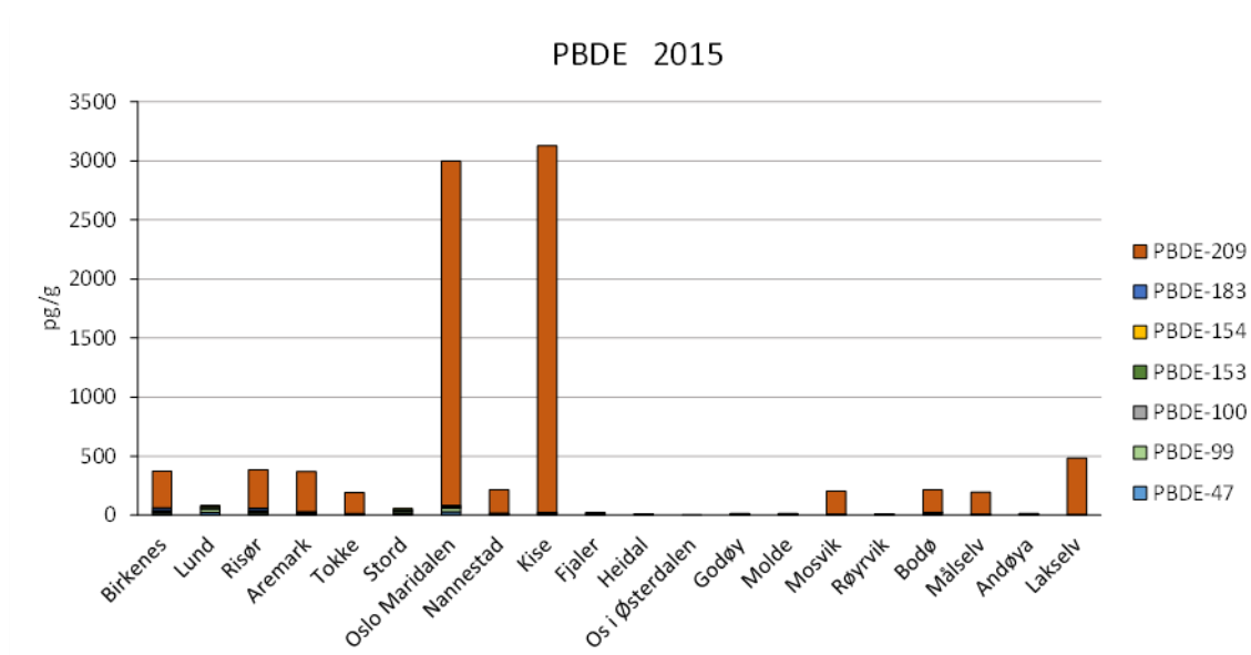
Figure 7: Distribution of selected PBDE congeners (including BDE-209) from the 2015 study.
