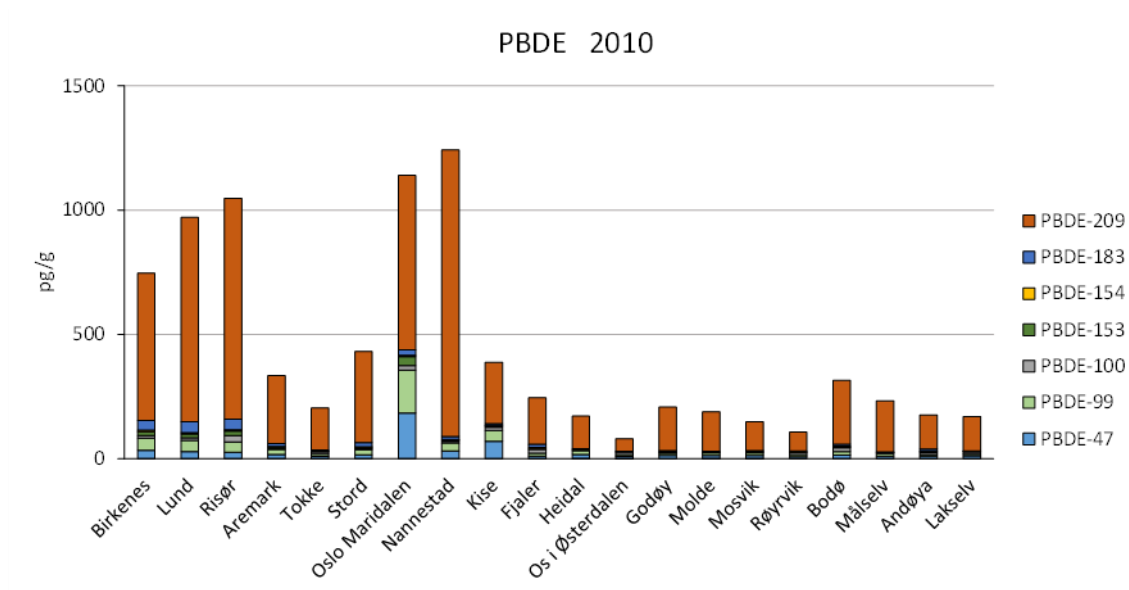
Figure 6: Distribution of selected PBDE congeners (including BDE-209) from the 2010 study.
