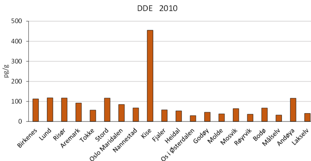
Figure 4: Distribution of p,p'-DDE from the 2010 study.
