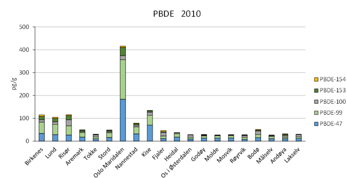
Figure 8: Distribution of selected PBDE congeners (without BDE-209) from the 2010 study.
