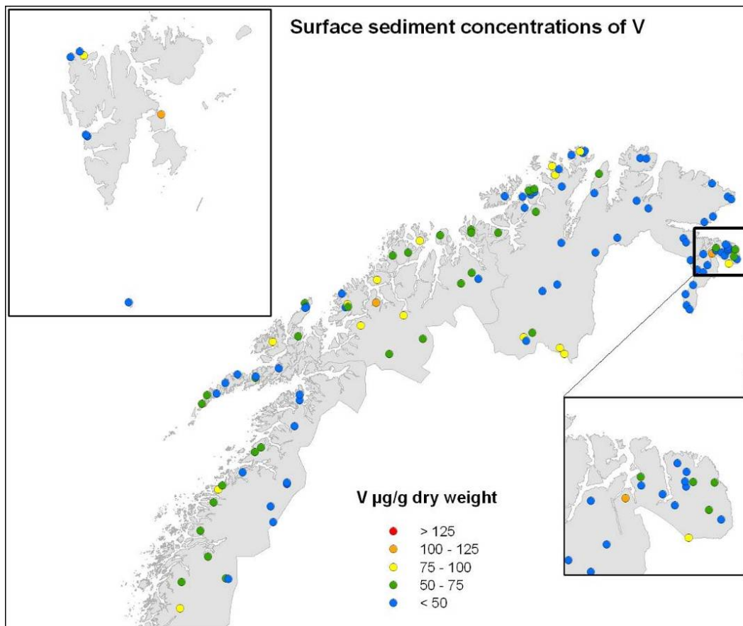
Figure 38. Concentrations (µg/g dw) of vanadium (V) in surface sediments from lakes on the mainland of Northern Norway and on Svalbard.
