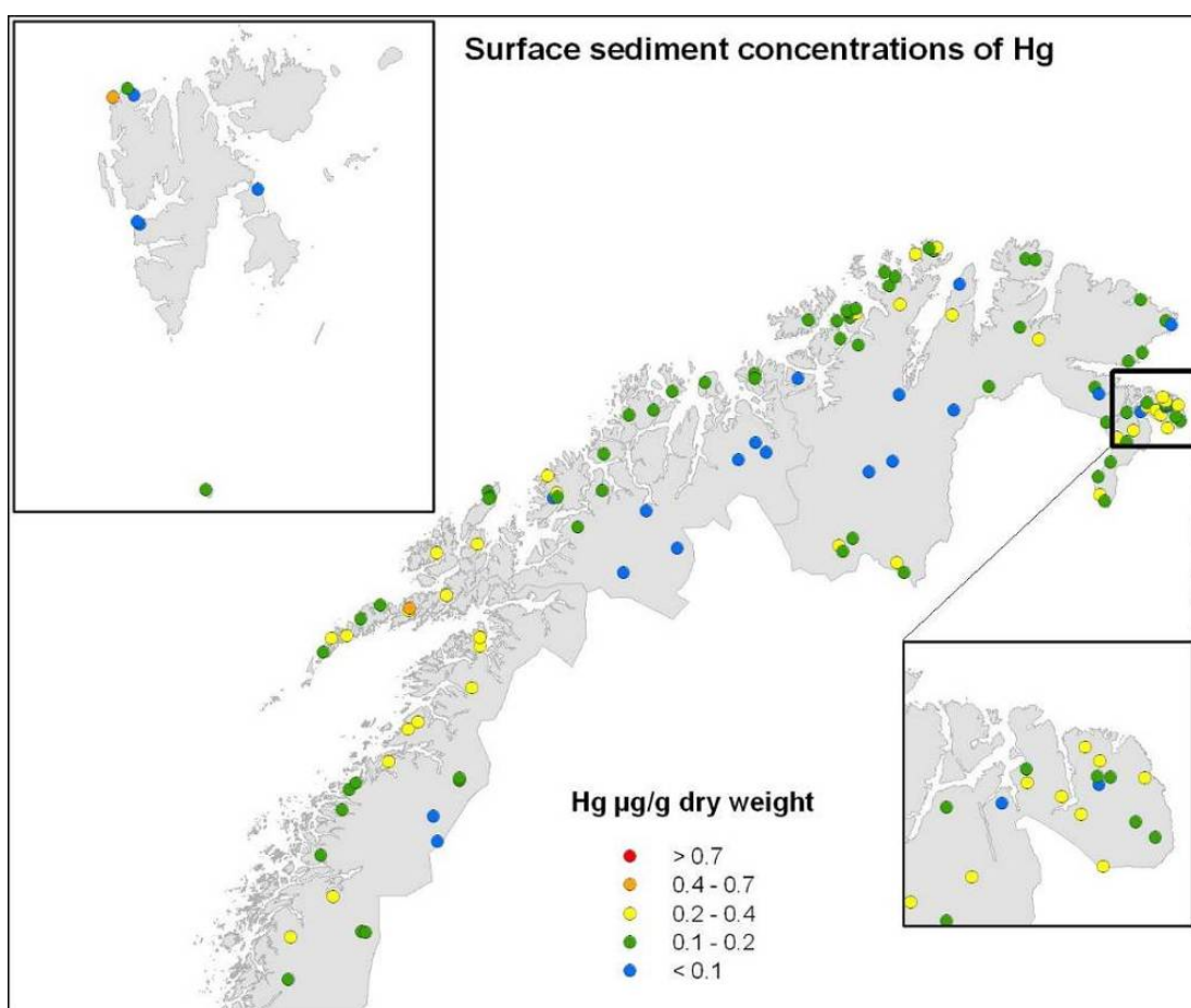
Figure 8. Concentrations (µg/g dw) of mercury (Hg) in surface sediments from lakes on the mainland of Northern Norway and on Svalbard.
