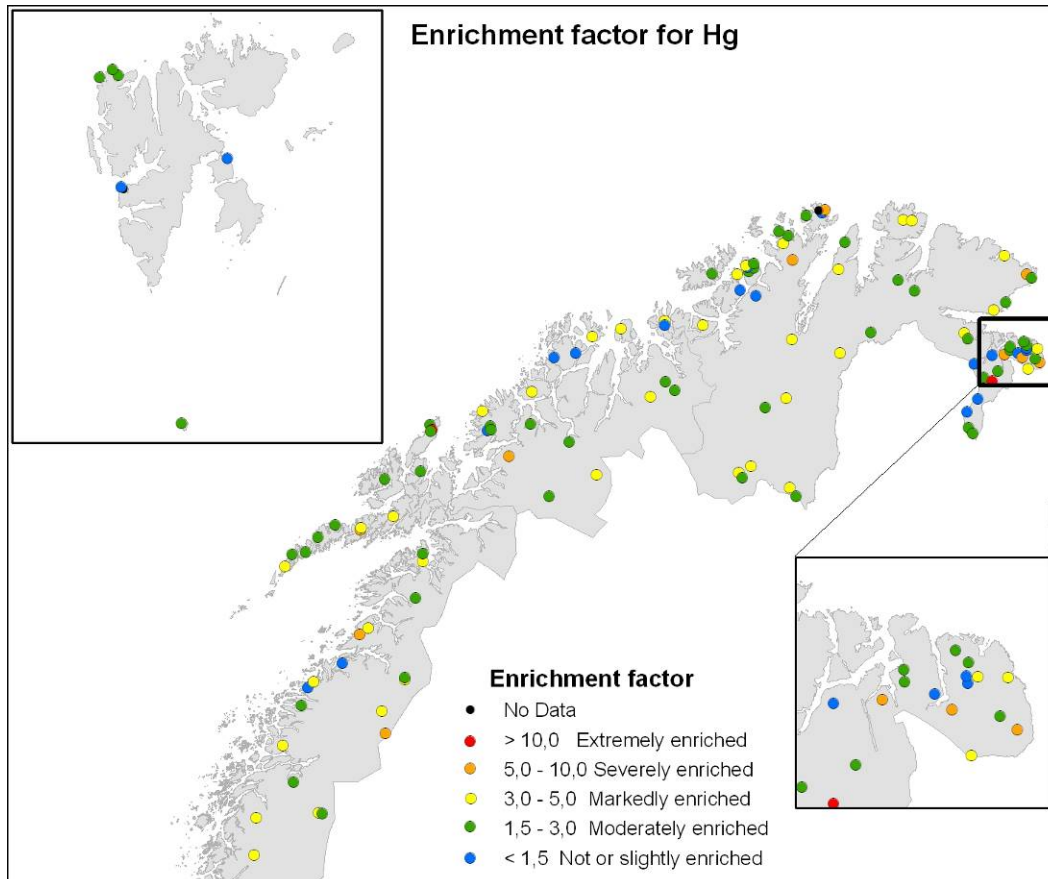
Figure 9. Enrichment factor for mercury (Hg) in surface sediment in lakes on the mainland of Northern Norway and on Svalbard.
