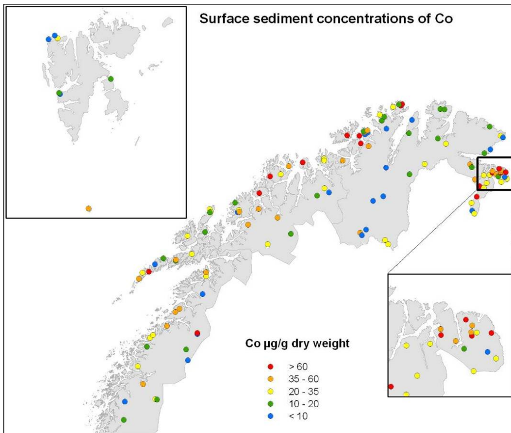
Figure 32. Concentrations (µg/g dw) of cobalt (Co) in surface sediments from lakes on the mainland of Northern Norway and on Svalbard.
