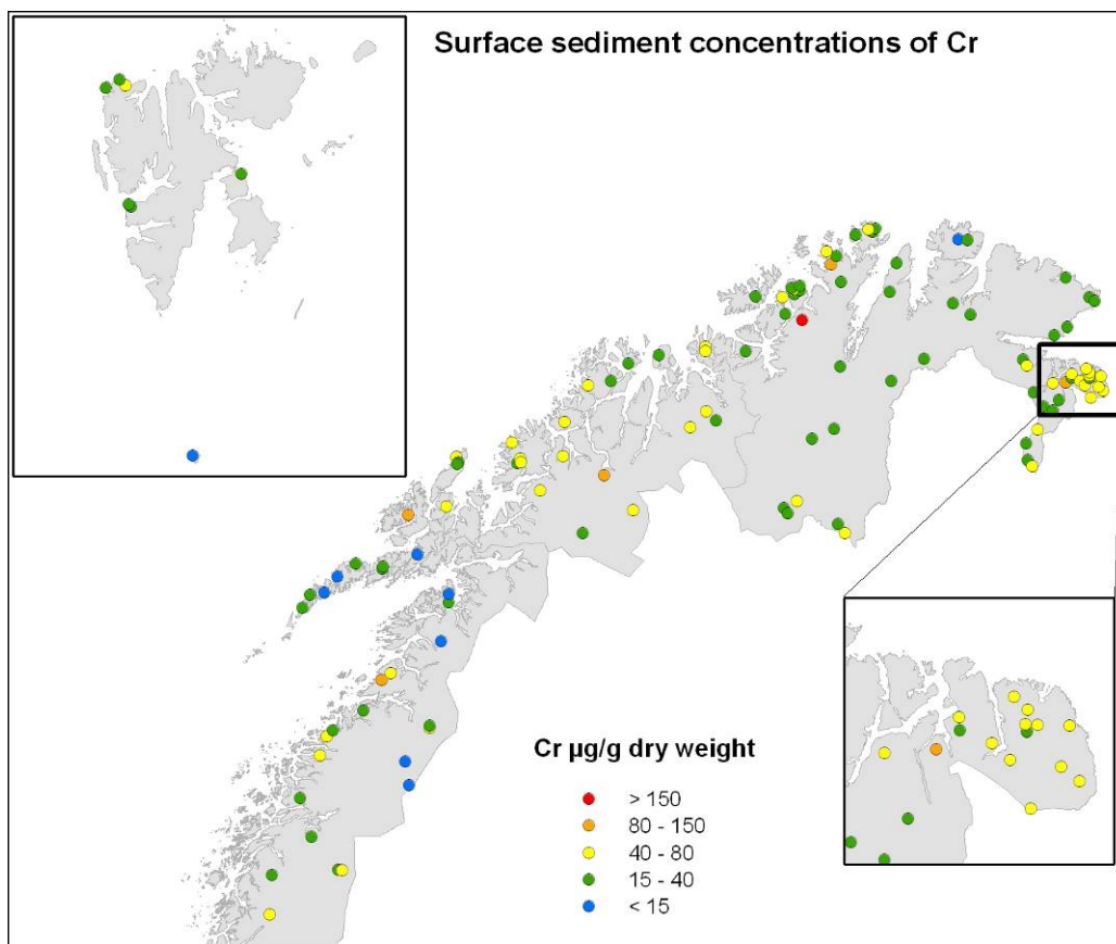
Figure 40. Concentrations (µg/g dw) of chromium (Cr) in surface sediment from lakes on the mainland of Northern Norway and on Svalbard.
