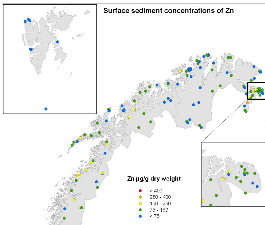
Figure 42. Concentrations (µg/g dw) of zinc (Zn) in surface sediments from lakes on the mainland of Northern Norway and on Svalbard.
