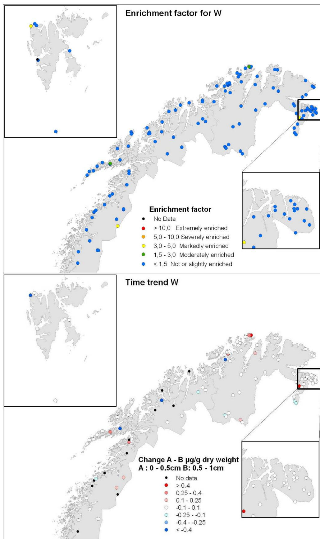
Figure 47. Enrichment factor for wolfram (W) in surface sediments (upper figure) and differences in concentrations ( \mu\text{g/g dw} ) of W between surface layer (0 - 0.5 cm) and subsurface layer (0.5 - 1.0 cm) (lower figure).
