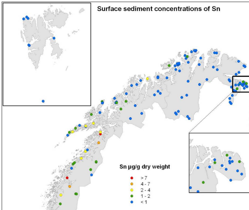
Figure 22. Concentrations (µg/g dw) of tin (Sn) in surface sediments from lakes on the mainland of Northern Norway and on Svalbard.
