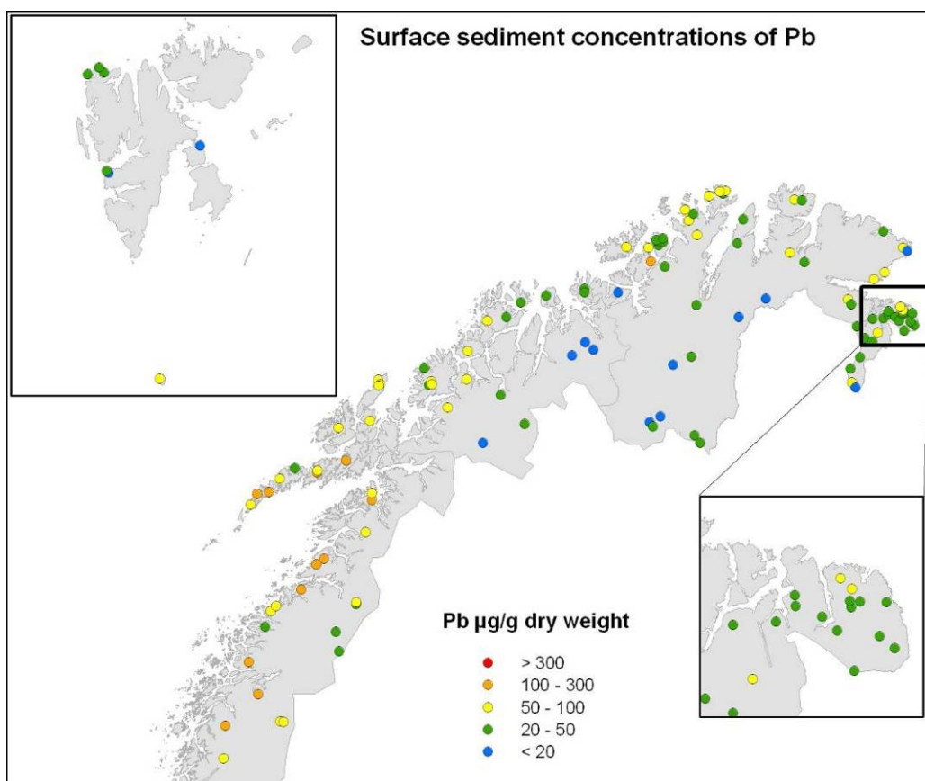
Figure 12. Concentrations (µg/g dw) of lead (Pb) in surface sediments from lakes on the mainland of Northern Norway and on Svalbard.
