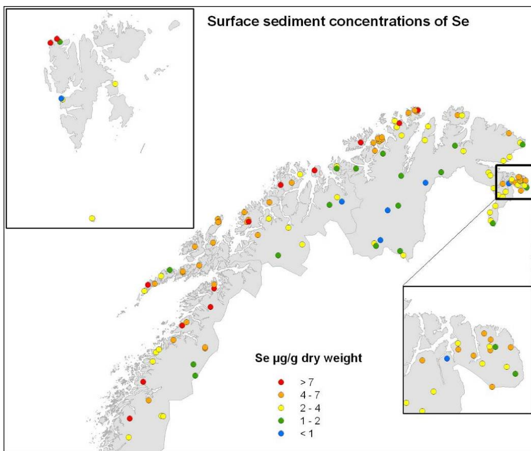
Figure 30. Concentrations (µg/g dw) of selenium (Se) in surface sediments from lakes on the mainland of Northern Norway and on Svalbard.
