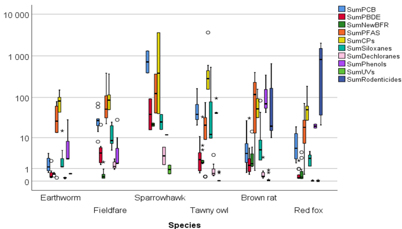
Figure 17: Box plot of the sum concentrations of the most dominating organic pollutant groups in the various biological samples. Concentrations are given in ng/g ww. The upper and lower boundaries of the box are representing the 25th and 75th percentile, the horizontal line in the box marks the median. Outliers are plotted as circle (1.5-3 IQR from end of box) or asterisk (>3 IQR from the end of the box). The whiskers represent the minimum and maximum values without outliers.
