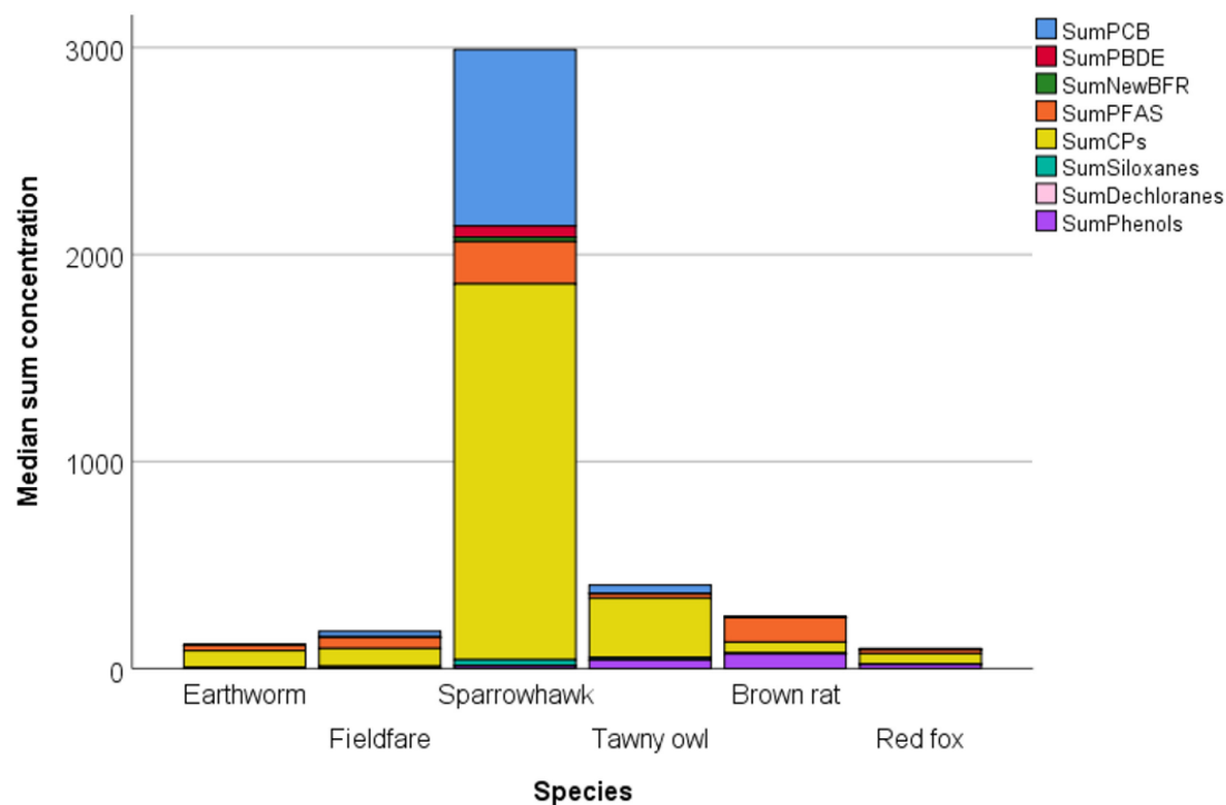
Figure 16: Organic pollutant groups in the various biota samples given by Median Sum concentrations (ng/g ww). Figure below shows percentage contribution of organic pollutant groups in the samples.
