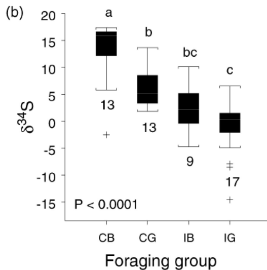
Fig. 2 Box plot showing the central 50% ( boxes ) and range ( lines ) of a \delta\text{D}_{\text{f-p}} and b \delta^{34}\text{S} for four foraging groups of raptors: coastal bird-eaters (CB), coastal generalists (CG), inland bird-eaters (IB), and inland generalists (IG). Letters above boxes indicate group membership and numbers below boxes indicate sample size. + An outlier value
