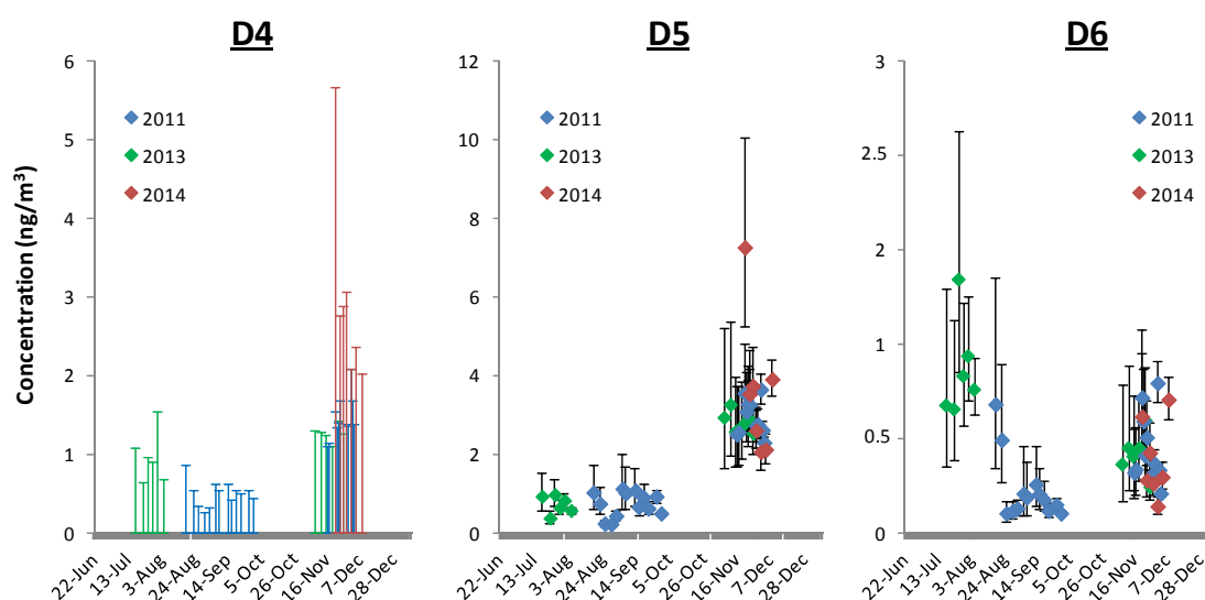
Figure 4.1: Measured concentrations of D4, D5 and D6 at Zeppelin in 2011 (blue), 2013 (green) and 2014 (red). Concentrations of D4 are reported as a range from non-detected to the upper limit detected. Concentrations of D5 and D6 are reported as a storage-corrected point-estimate with a range representing the 95% confidence interval of the storage correction.
