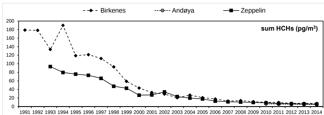
Figure 3.3: Annual mean concentrations of sum HCHs (pg/m³) in air.
