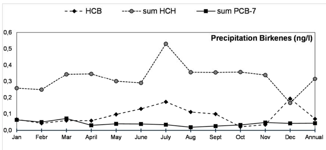
Figure 3.21: Monthly and annual mean concentrations (ng/l) of HCB, sum HCHs and sum PCB-7 in precipitation at Birkenes, 2014.
