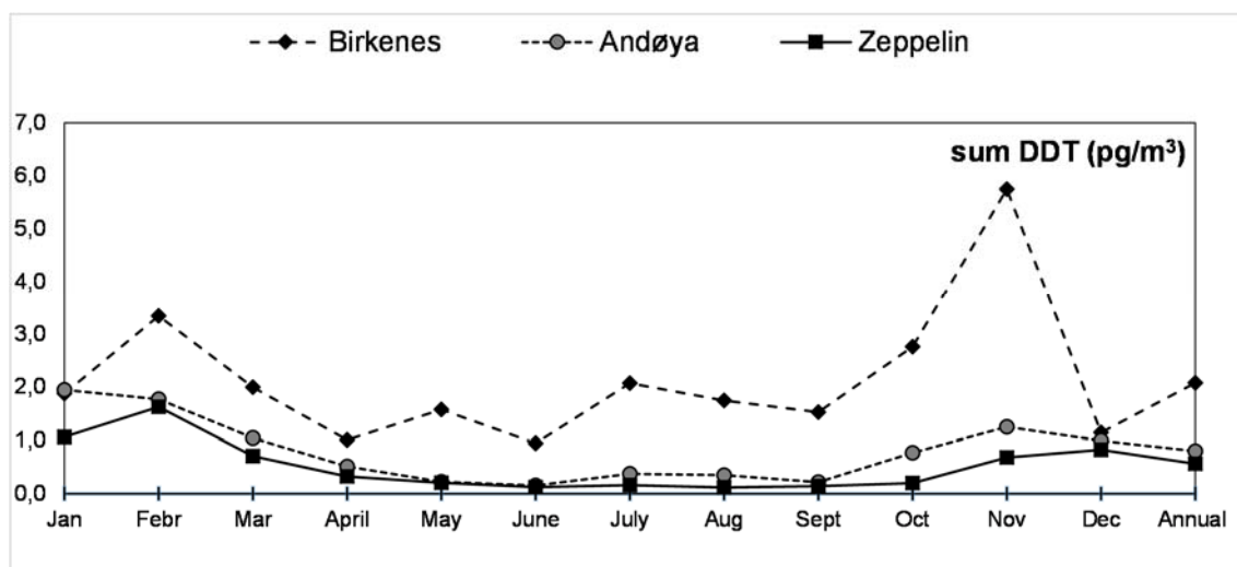
Figure 3.6: Monthly and annual mean concentrations (pg/m³) of sum DDTs in air for 2014.
