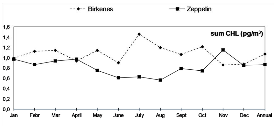
Figure 3.8: Monthly and annual mean concentrations (pg/m³) of sum CHLs in air for 2014.
