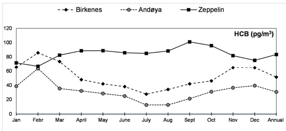
Figure 3.2: Monthly and annual mean concentrations (pg/m 3 ) of HCB in air for 2014.
