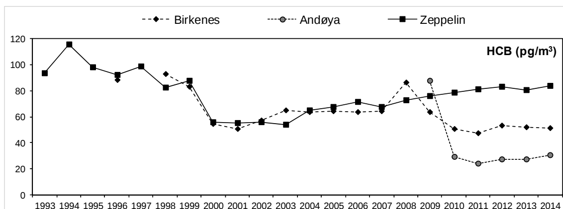
Figure 3.1: Annual mean concentrations of HCB (pg/m 3 ) in air.
