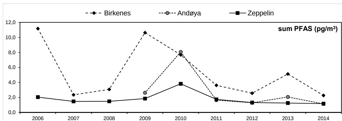
Figure 3.18: Annual mean concentrations of sum PFAS (pg/m 3 ) in air.
