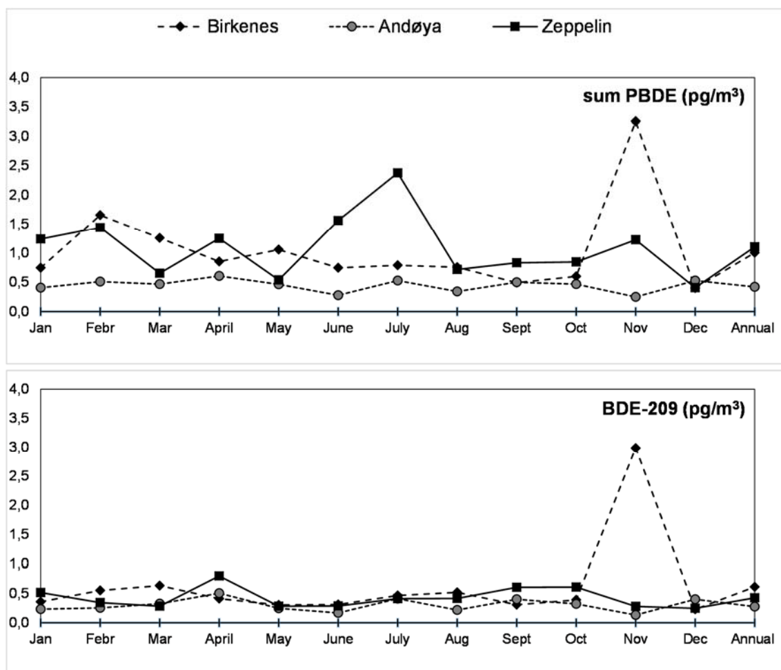
Figure 3.12: Monthly and annual mean concentrations (pg/m³) of sum PBDEs and BDE-209 in air for 2014.
