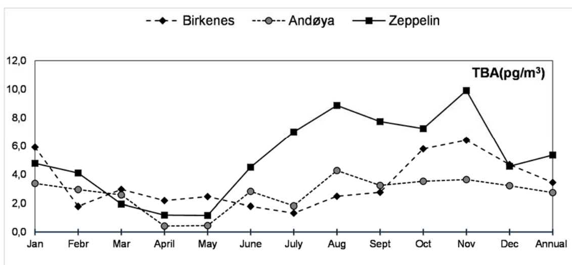
Figure 3.14: Monthly and annual mean concentrations (pg/m³) of TBA in air for 2014.
