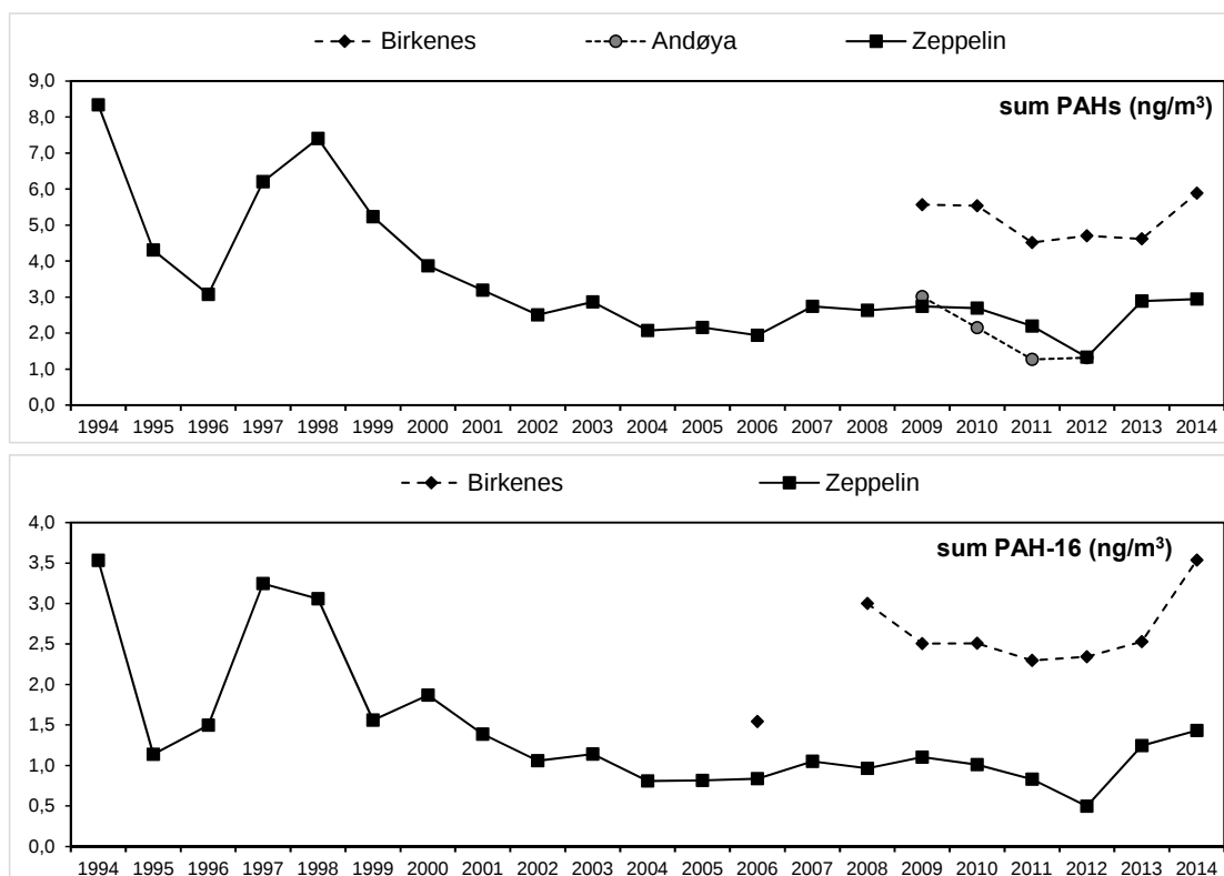
Figure 3.16: Annual mean concentrations of sum PAHs and sum PAH-16 (ng/m³) in air.
