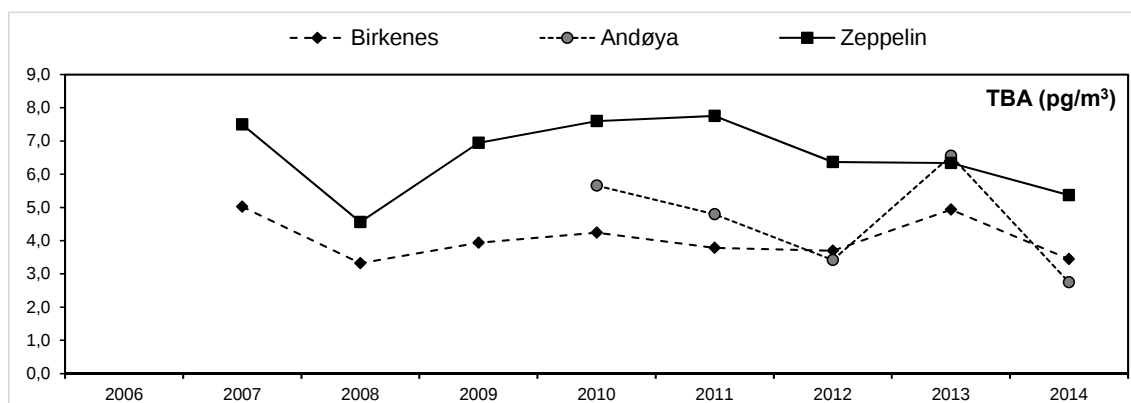
Figure 3.13: Annual mean concentrations of TBA (pg/m³) in air.
