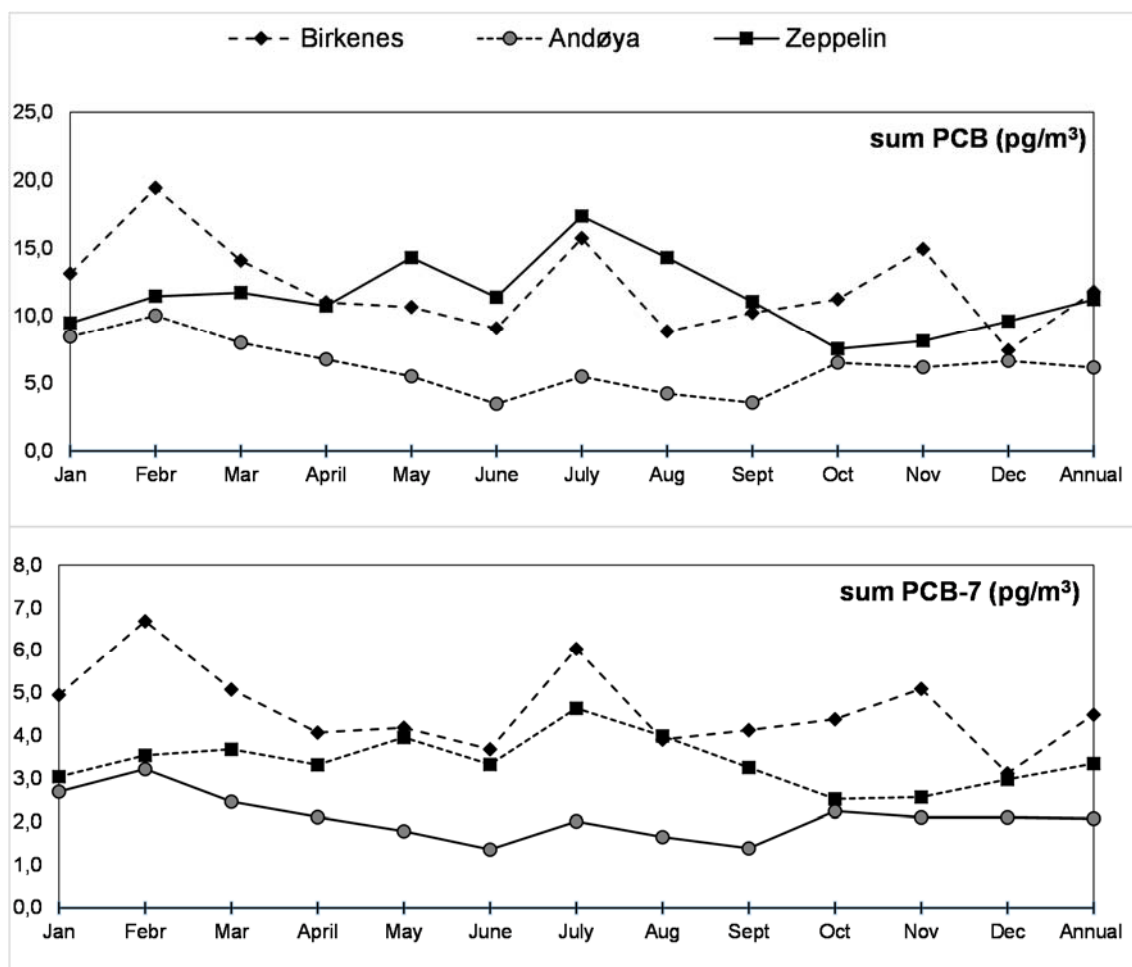
Figure 3.10: Monthly and annual mean concentrations (pg/m³) of sum PCBs and sum PCB-7 in air for 2014.
