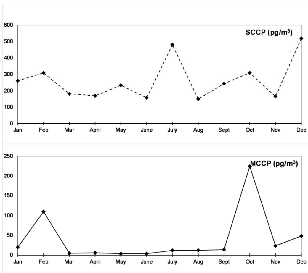
Figure 4.3: Monthly mean concentrations (pg/m³) of SCCPs and MCCPs in air at Zeppelin, 2014.
