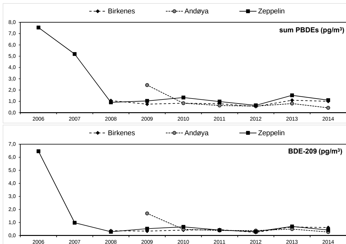
Figure 3.11: Annual mean concentrations of sum PBDEs and BDE-209 ( \text{pg}/\text{m}^3 ) in air.
