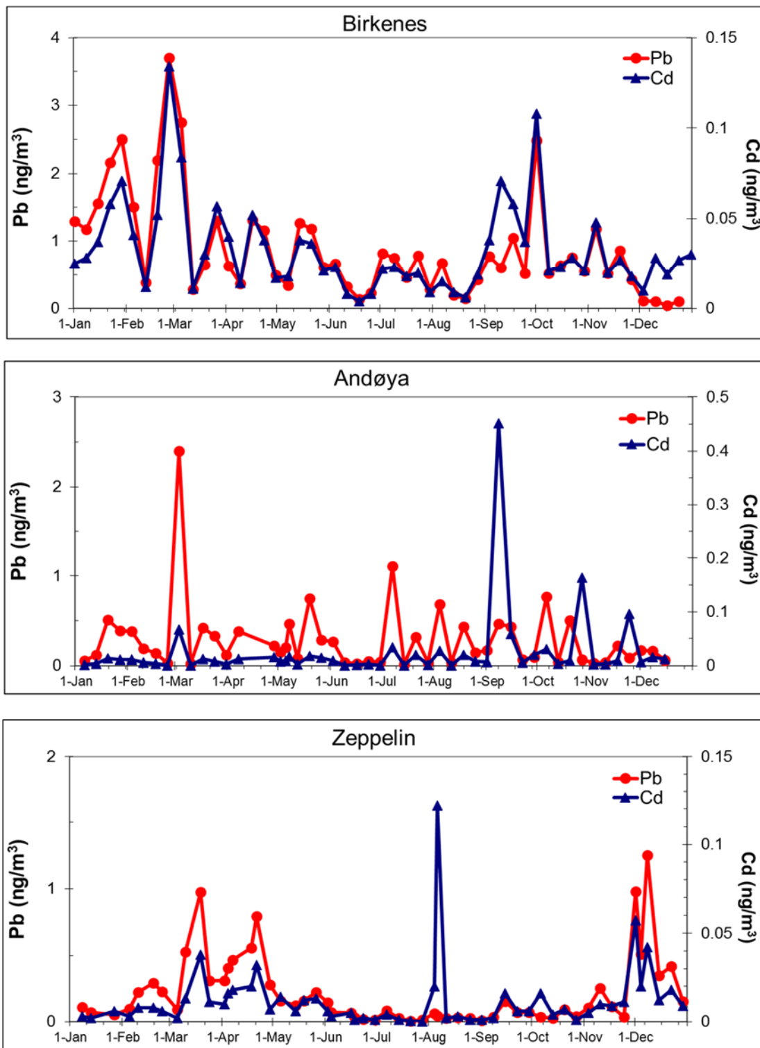
Figure 2.3: Weekly concentrations of lead and cadmium in air at Norwegian background stations in 2014, Unit: ng/m 3 .
