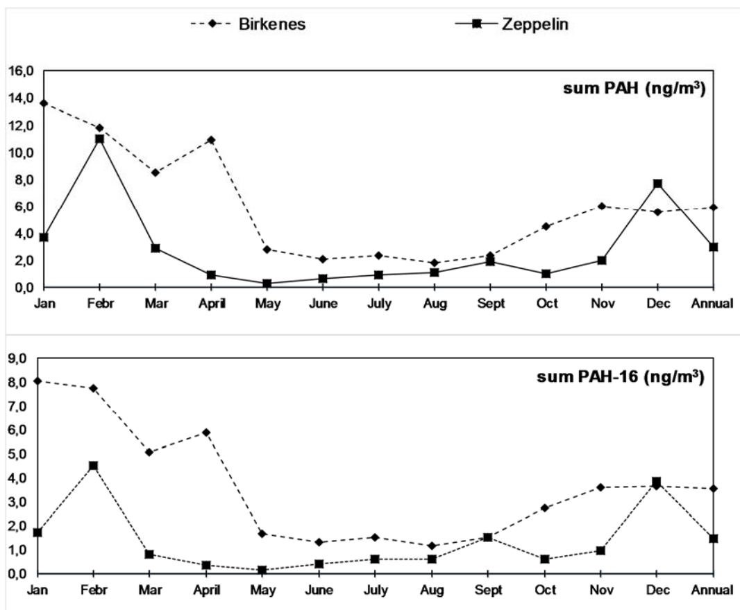
Figure 3.17: Monthly and annual mean concentrations (ng/m³) of sum PAHs and sum PAH-16 in air for 2014.
