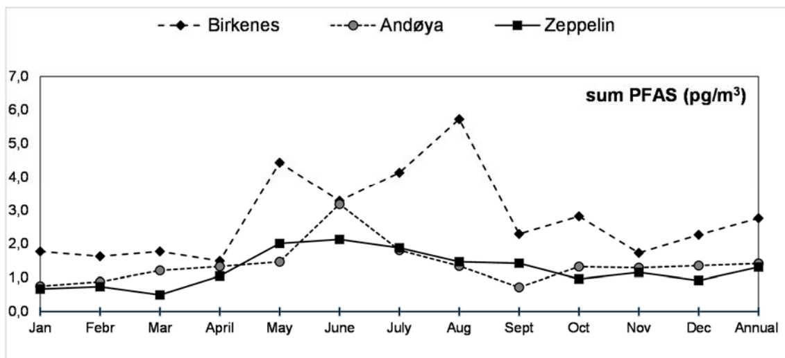
Figure 3.19: Monthly and annual mean concentrations (pg/m³) of sum PFAS in air for 2014.
