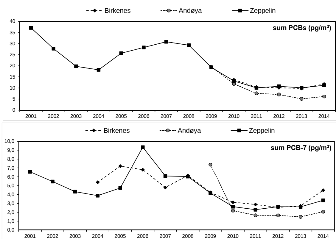
Figure 3.9: Annual mean concentrations of sum PCBs and sum PCB-7 ( \text{pg}/\text{m}^3 ) in air.
