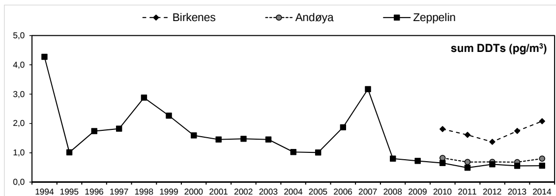
Figure 3.5: Annual mean concentrations of sum DDTs (pg/m 3 ) in air.
