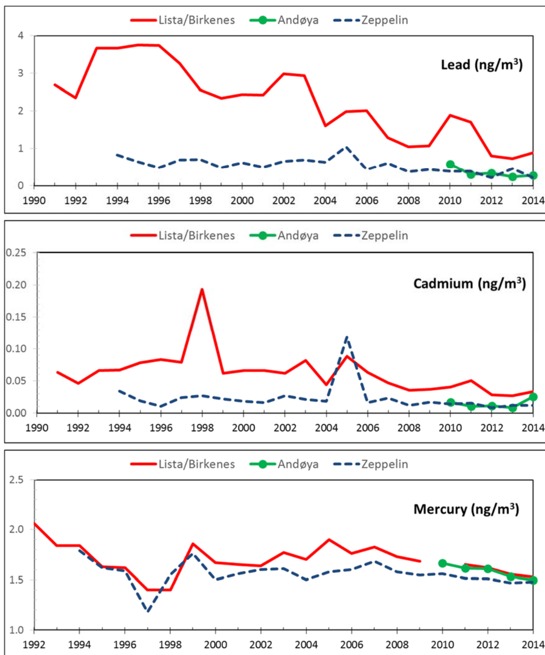
Figure 2.4: Time series of annual mean average concentrations of lead, cadmium and mercury in air and aerosols, 1991-2014, Unit: ng/m 3 (note that the y-axis for mercury begins at 1.0 ng/m 3 ).
