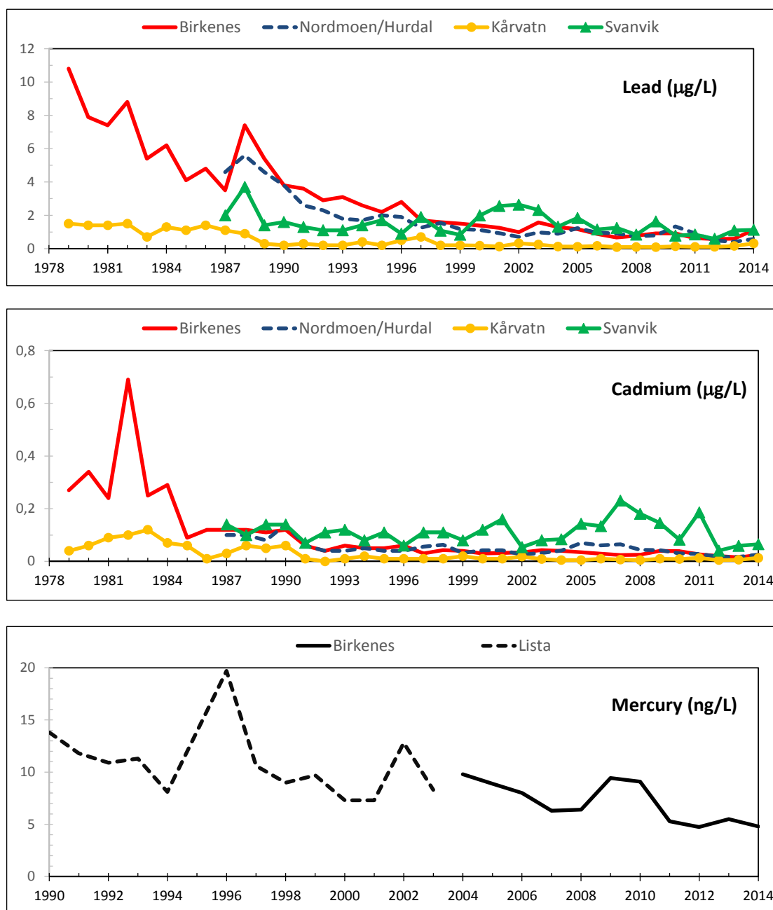
Figure 2.2: Time series of annual volume weighted mean of lead, cadmium and mercury in precipitation at Norwegian background stations.
