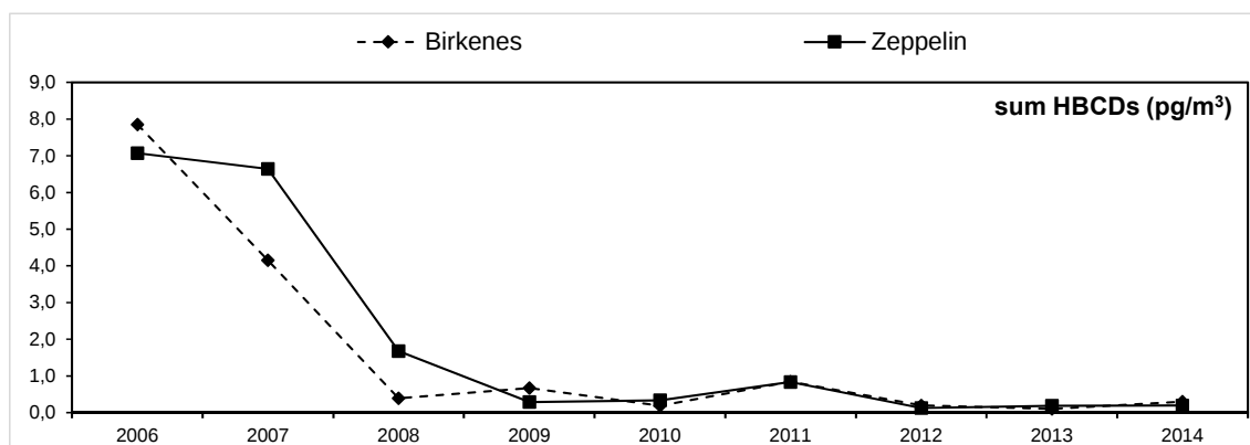
Figure 3.15: Annual mean concentrations of sum HBCDs (pg/m³) in air.
