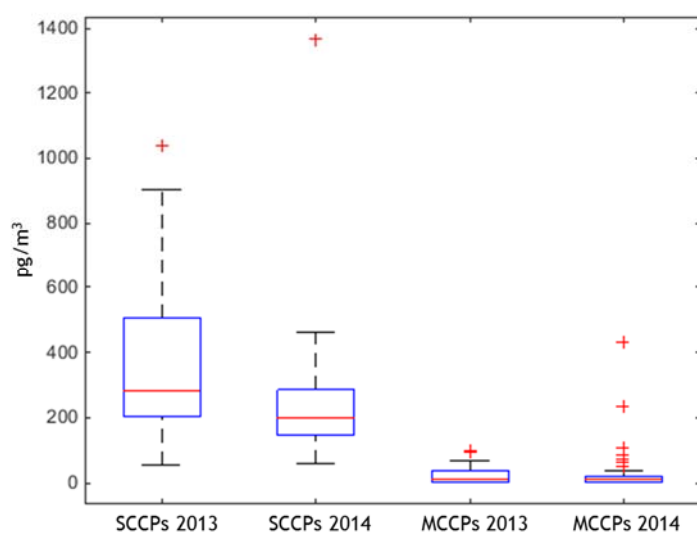
Figure 4.2: Box-whisker plot representing the annual mean concentrations and distribution of SCCPs and MCCPs in air at Zeppelin in 2013 and 2014 respectively.
