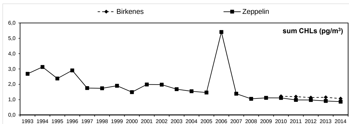
Figure 3.7: Annual mean concentrations of sum CHLs (pg/m³) in air.
