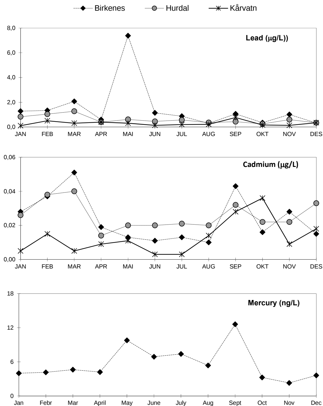
Figure 2.1: Monthly average volume weighted mean concentrations of lead, cadmium and mercury in precipitation in 2014.
