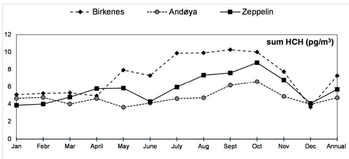
Figure 3.4: Monthly and annual mean concentrations (pg/m³) of sum HCHs in air for 2014.
