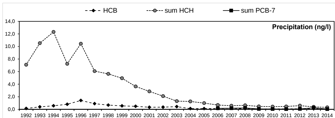
Figure 3.20: Annual mean concentrations of HCB, sum HCHs and sum PCB-7 (ng/l) in precipitation.
