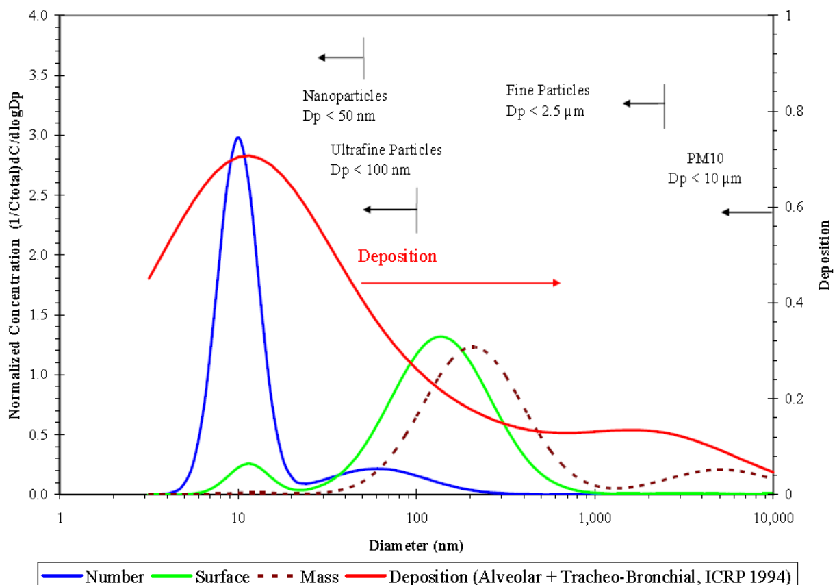
Figure 3 - Typical particle distributions and deposition (Kittelson, Watts et al. 2004)
