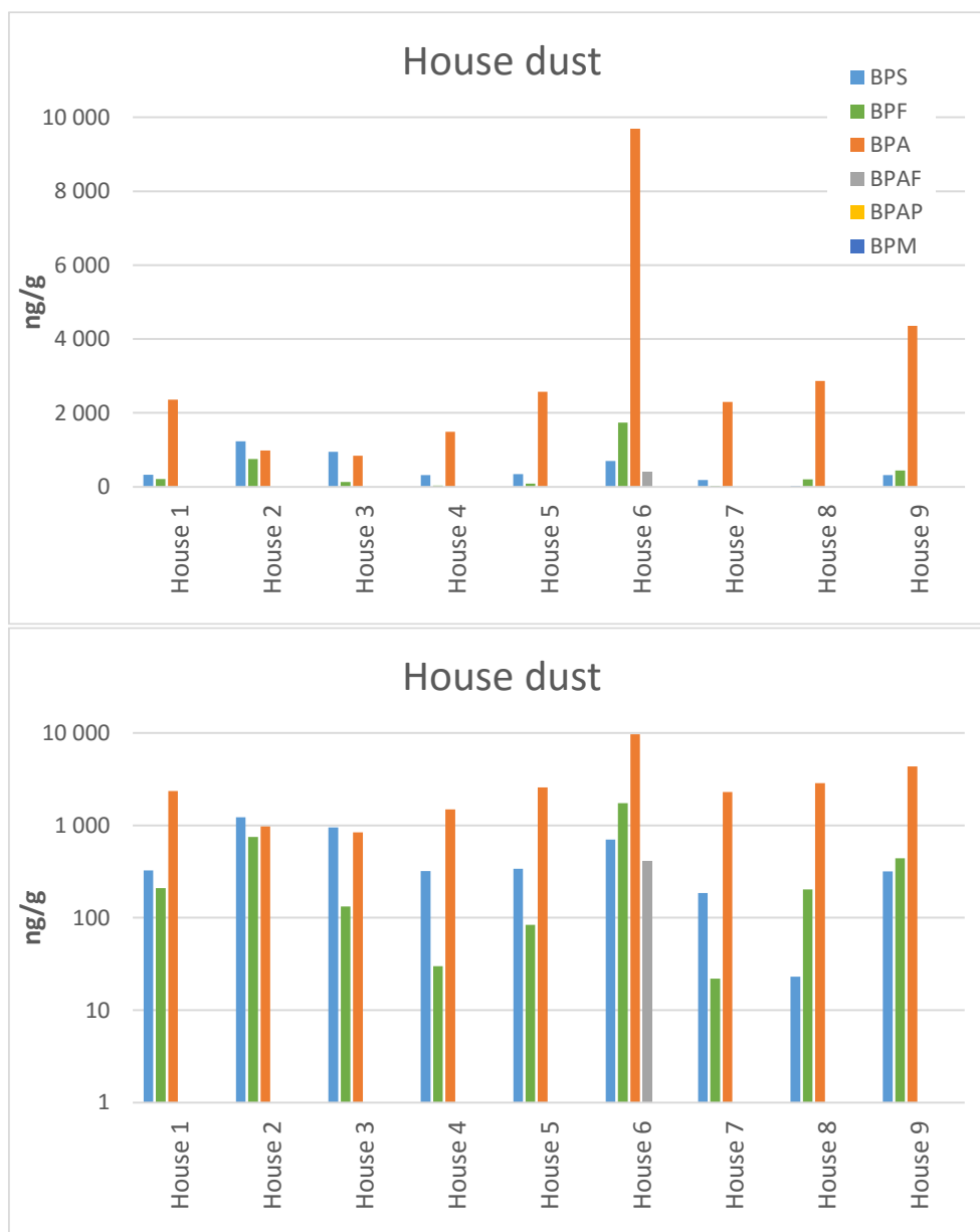
Figure 7: House dust concentration of bisphenols. Concentration given in ng/g, linear scale top figure, logarithmic scale bottom figure.
