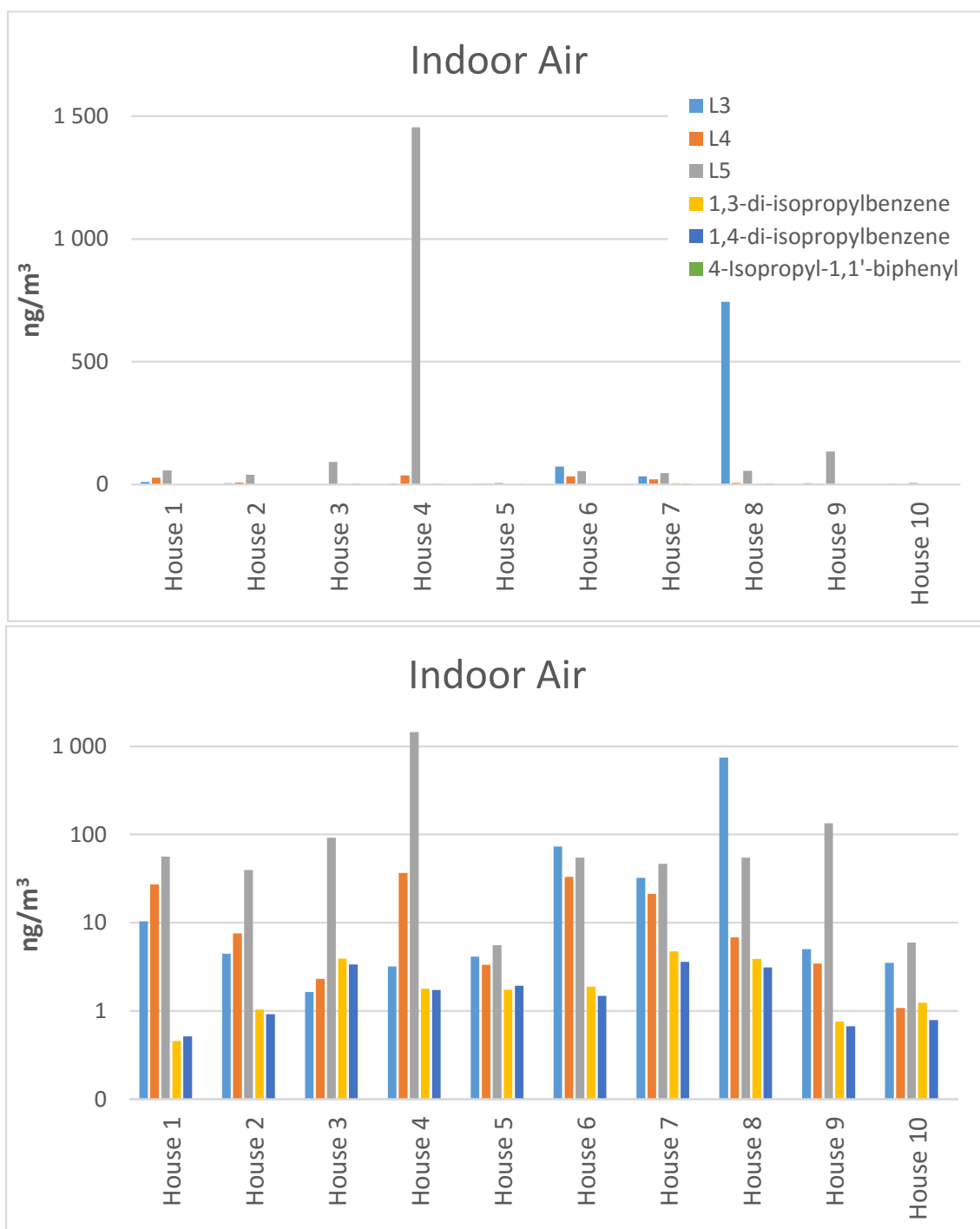
Figure 4: Indoor air concentration of linear siloxanes and some volatile aromatics. Concentration given in \text{ng}/\text{m}^3 , linear scale top figure, logarithmic scale bottom figure.
