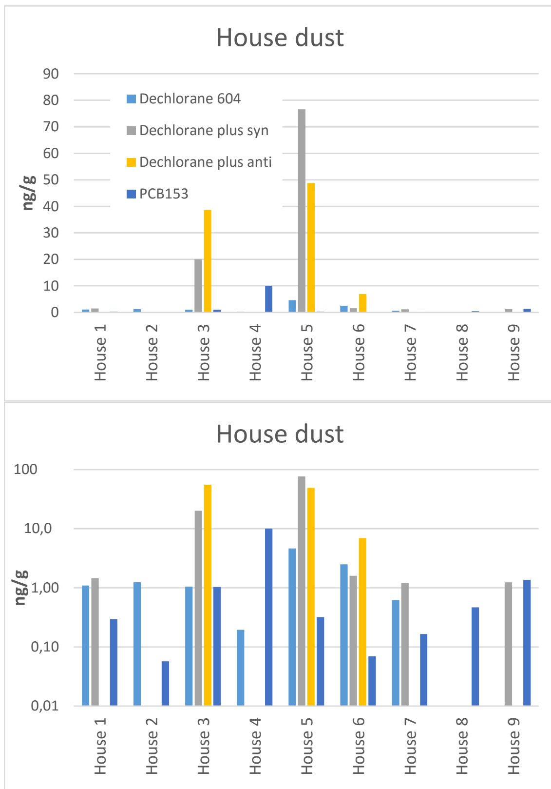
Figure 6: House dust concentration of dechloranes and PCB-153. Concentration given in ng/g, linear scale top figure, logarithmic scale bottom figure.
