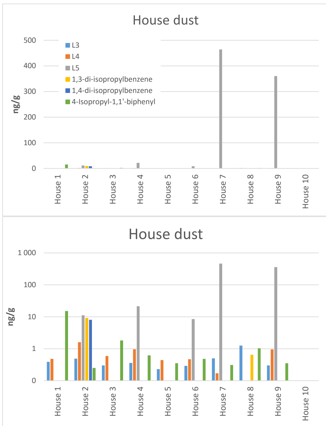
Figure 3: House dust concentration of linear siloxanes and some volatile aromatics. Concentration given in ng/g, linear scale top figure, logarithmic scale bottom figure.
